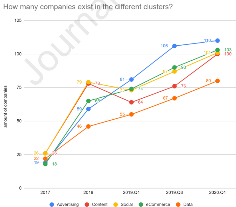
Fig. 4. Category clusters
