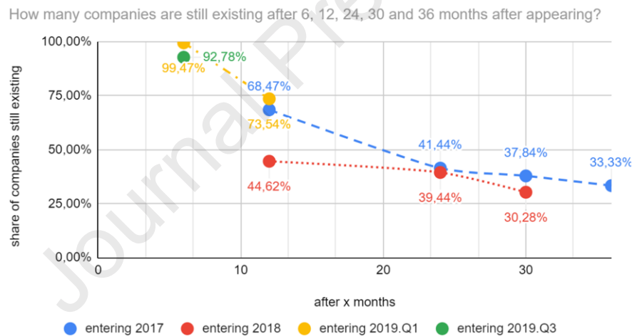
Fig. 3. Cohort analysis
